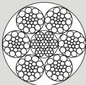
6x26 WS
