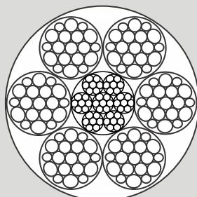
6x19 WGT
